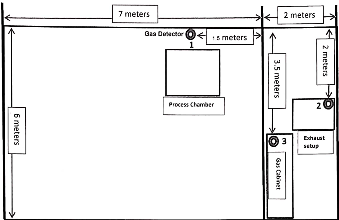
Fig. 1 Detail Lab Schematic Diagram for Gas Leak Detection System for Three Collection Points
